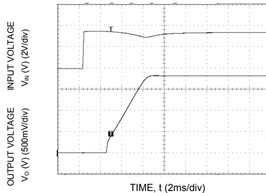
Figure 18. Typical Start-up Using Input Voltage ( V_{IN} = 3.3V , I_o = I_{o,max} ).
